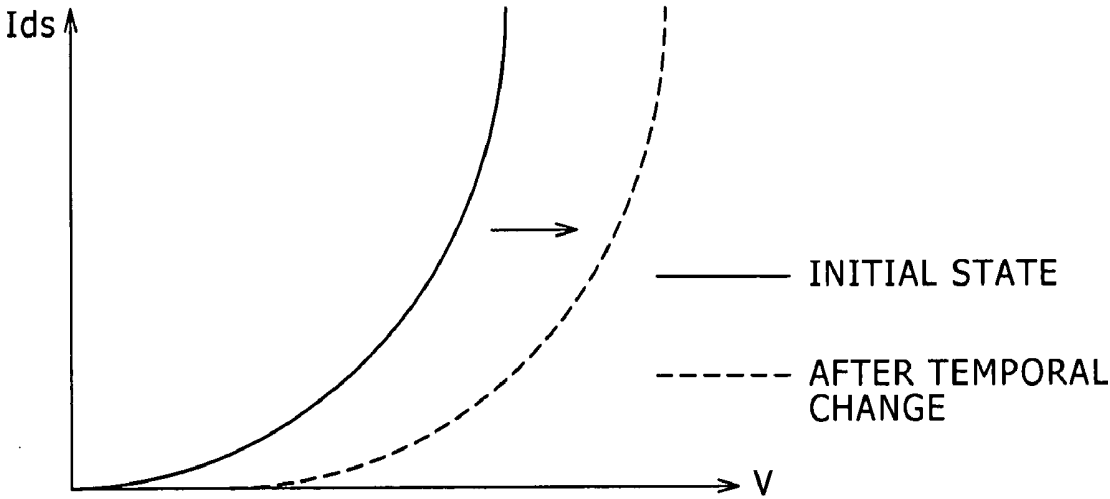
I-V CHARACTERISTICS OF OLED
